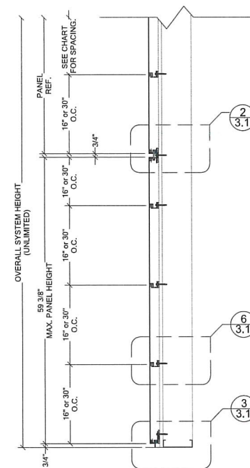
3 2.4 REF: NONE SCALE: 1"=1'-0" PANELS SECTION - B - 3MM PLATE RAIN SCREEN
