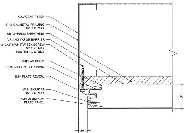
4 3.2 JAMB TERMINATION REF: NONE SCALE: 6"=1'-0"
