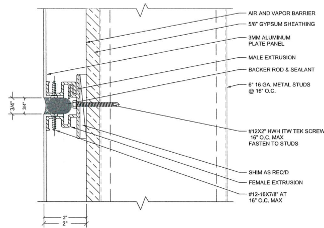
2 TYP. HORIZONTAL JOINT REF: NONE SCALE: 6"=1'-0"
