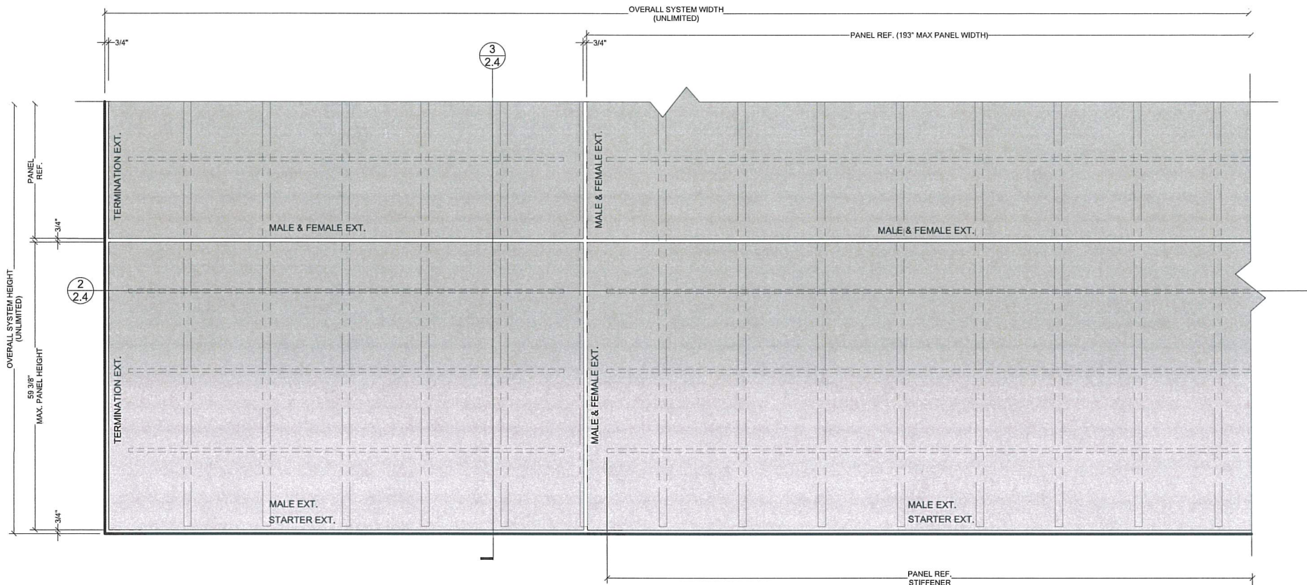
1 2.4 REF: NONE SCALE: 1"=1'-0" PANELS ELEVATION - 3MM PLATE RAIN SCREEN
