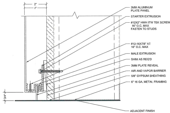
3 3.2 TYP. BASE TERMINATION REF: NONE SCALE: 6"=1'-0"
