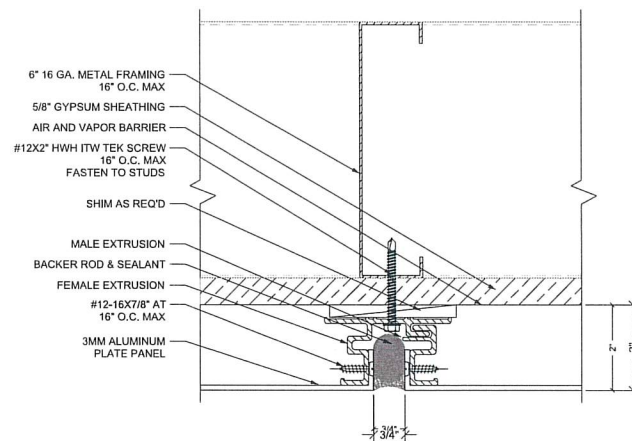
5 TYP. VERTICAL JOINT REF: NONE SCALE: 6"=1'-0"
