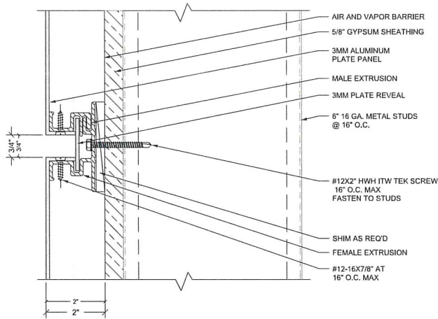
2 3.2 TYP. HORIZONTAL JOINT REF: NONE SCALE: 6"=1'-0"
