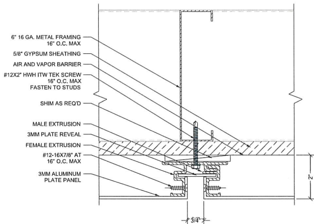
5 3.2 TYP. VERTICAL JOINT REF: NONE SCALE: 6"=1'-0"
