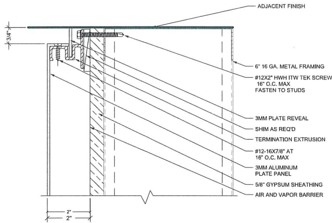
1 3.2 HEAD TERMINATION REF: NONE SCALE: 6"=1'-0"
