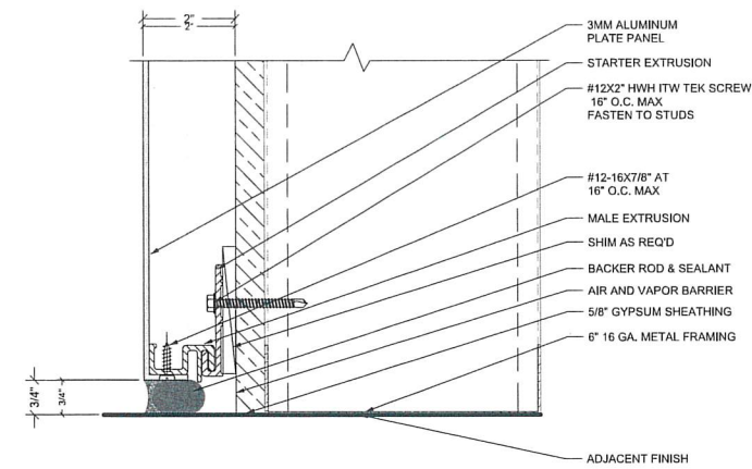
3 TYP. BASE TERMINATION REF: NONE SCALE: 6"=1'-0"
