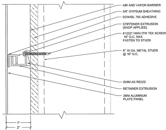
6 3.2 STIFFENER/RETAINER DETAIL REF: NONE SCALE: 6"=1'-0"
